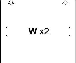
573x474x15mm
